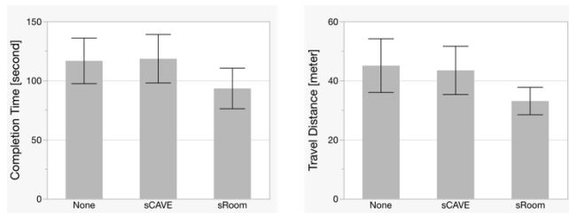
Figure 2. Mean data of completion time (left) and travel distance (right). Error bars indicate confidence intervals ( CI = .95 )
