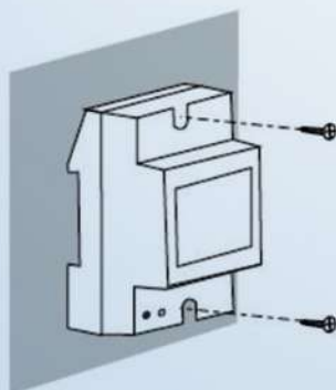
Direct wall-mounted
