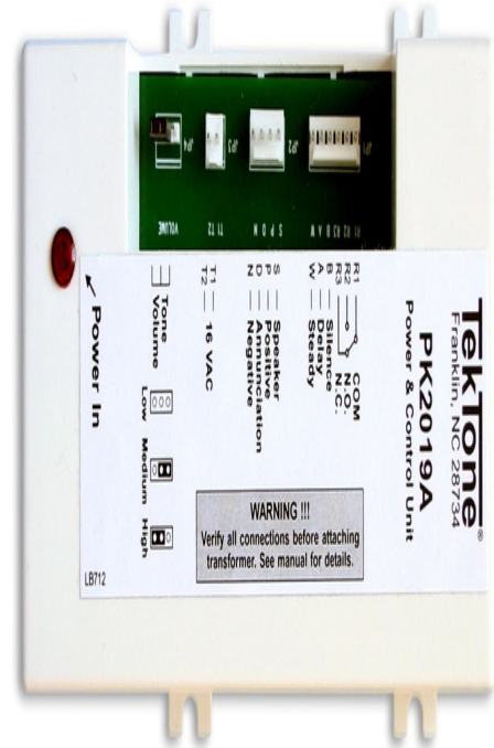
PK2019A Power and Control Unit
