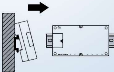
DIN-Rail mounted
