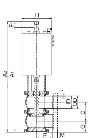
Shut-off valve
