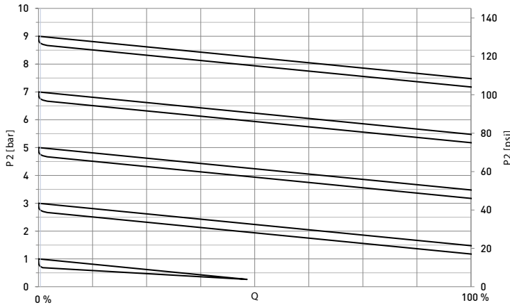
100% corresponds to a flow velocity of 6.6 ft/s
