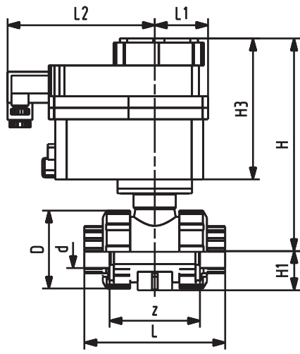
Socket/threaded
