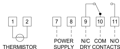
Figure 2: DLC Wiring
