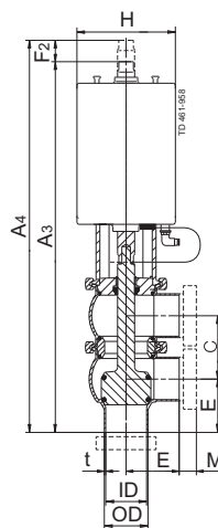
Change-over valve
