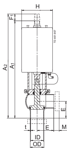
Shut-off valve
