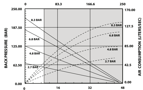
FLOW RATE - LITERS PER MINUTE (LPM)
