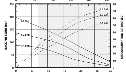
PERFORMANCE BASED ON 30wt. OIL (100cSt) AT 40°C TEMPERATURE CYCLE PER MINUTE (CPM)
