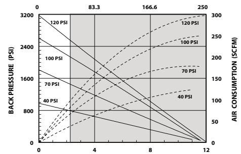
FLOW RATE - GALLONS PER MINUTE (GPM)
