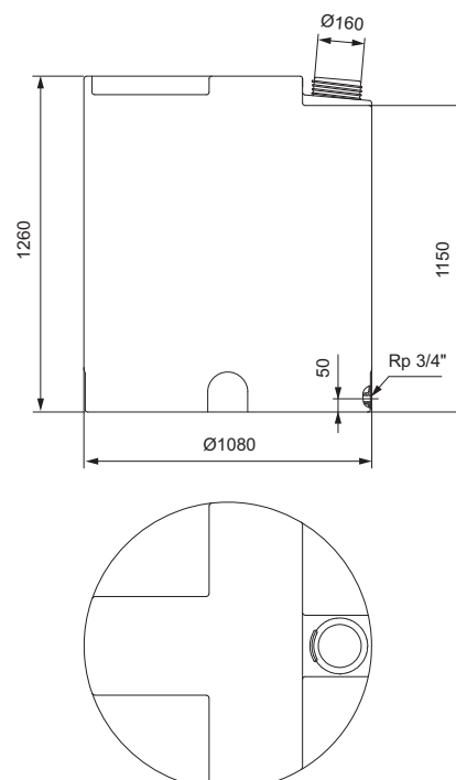
Fig. 55 Cylindrical tank, 1000 litres
