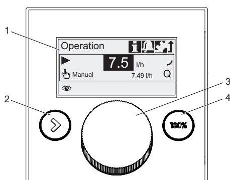
Fig. 7 Operating elements DDA and DDC
