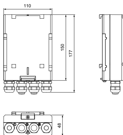
Fig. 28 E-box, dimensions
