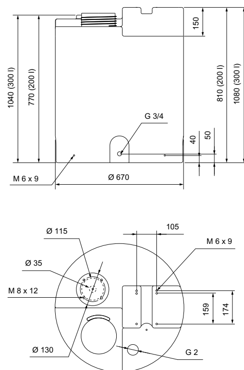
Fig. 53 Cylindrical tank, 200 and 300 litres
