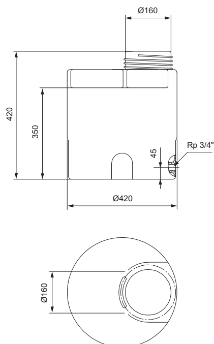
Fig. 51 Cylindrical tank, 40 litres
