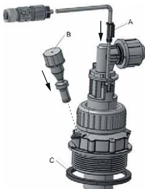
Fig. 35 Emission protection kit
