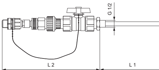
Fig. 40 Injection unit with removable injection pipe
