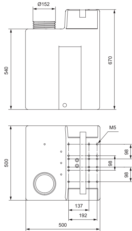
Fig. 49 Square tank, dimensions
