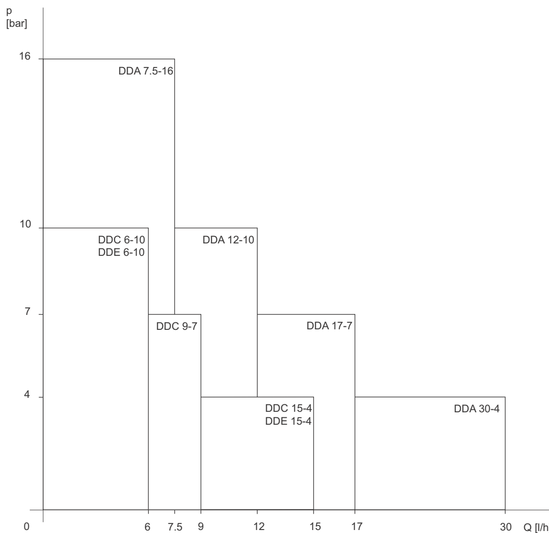
Fig. 1 Performance range
