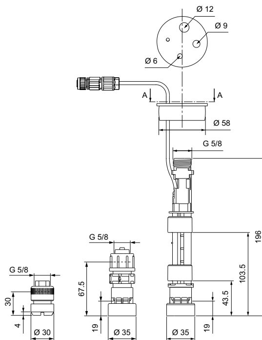
Fig. 31 Foot valves: stainless-steel (left), PE or PVDF (centre and right)
