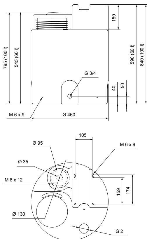
Fig. 52 Cylindrical tank, 60 and 100 litres
