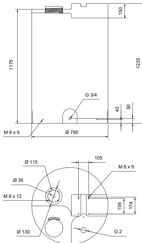
Fig. 54 Cylindrical tank, 500 litres
