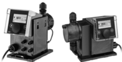
Fig. 6 Two of three possible control cube positions
