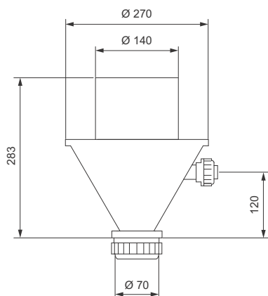
Fig. 57 Dissolving hopper, dimensions
