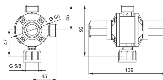
Fig. 43 Multi-function valve
