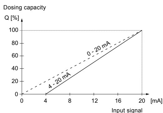
Fig. 10 0/4-20 mA control
