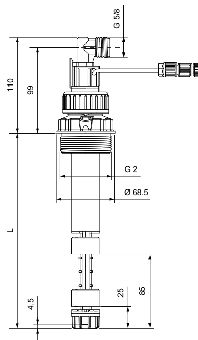
Fig. 33 Rigid suction lance
