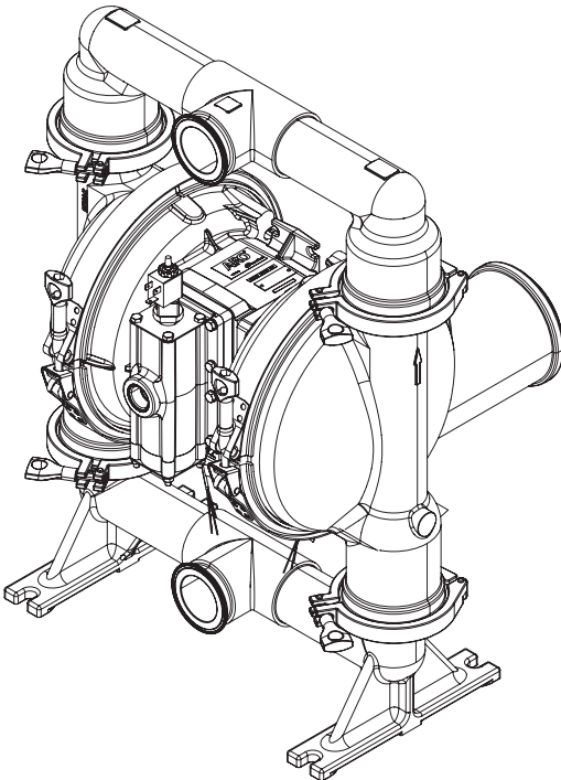
SD20R-XXX-XXX-BXXX Figure 1
