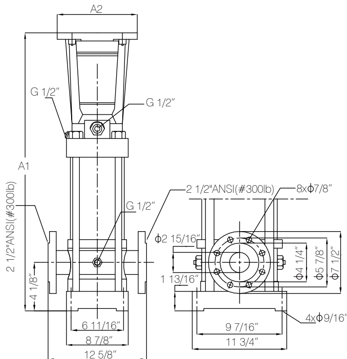
Pump Dimensions
