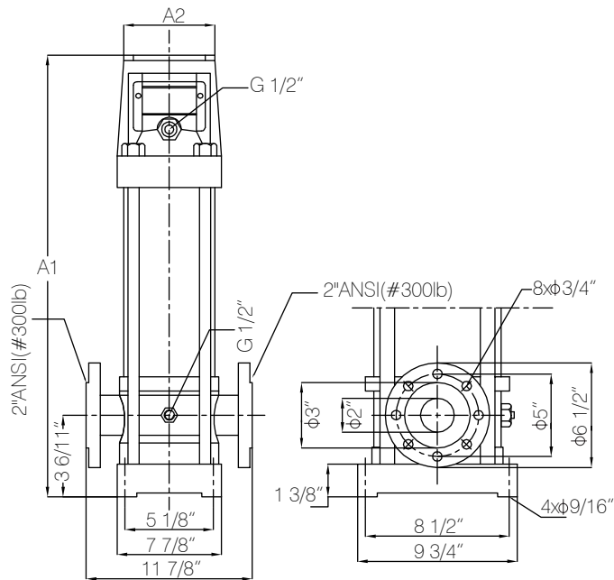
Pump Dimensions
