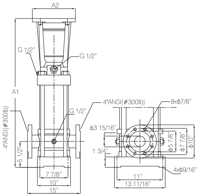
Pump Dimensions
