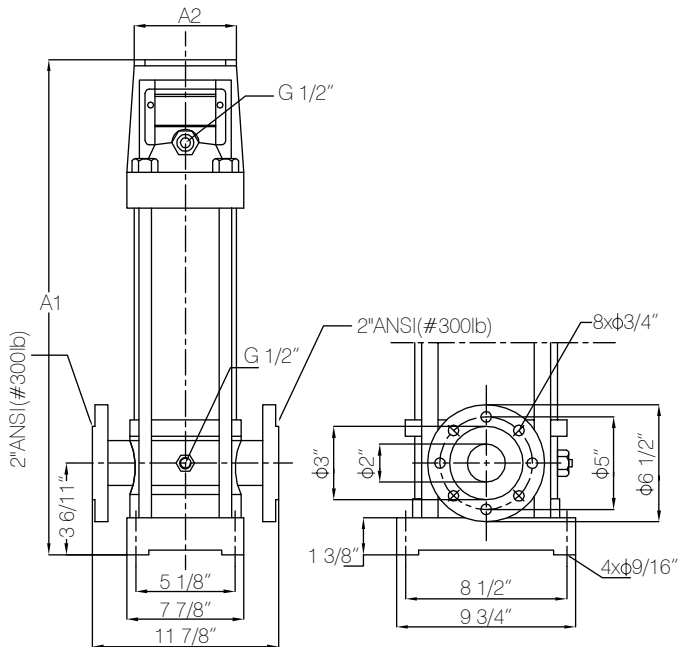
Pump Dimensions
