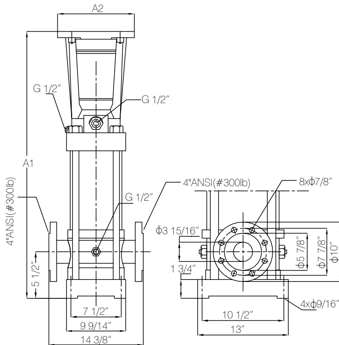
Pump Dimensions
