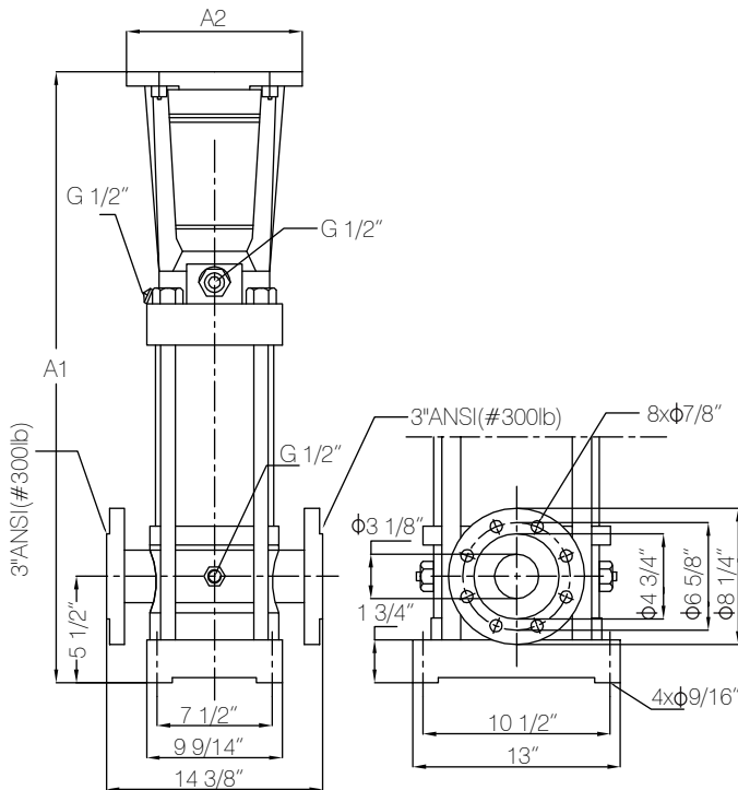
Pump Dimensions
