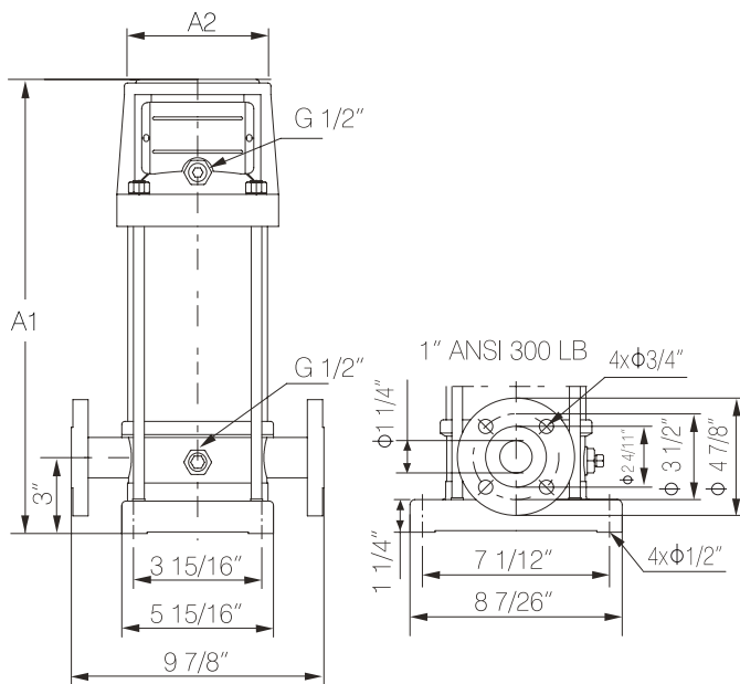
Pump Dimensions
