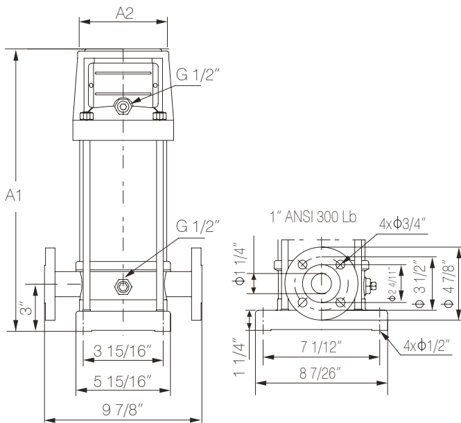
Pump Dimensions
