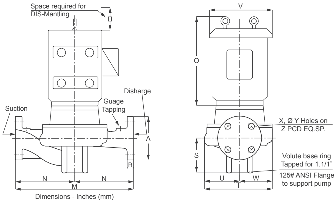
Pump Dimensional Data
