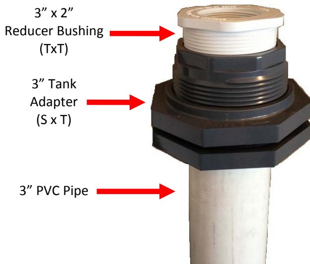
Stand-Pipe Example
