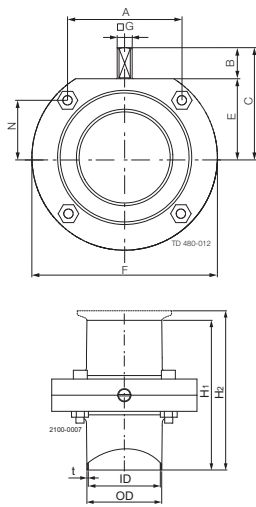
Fig. 1. Dimensions - valve.
