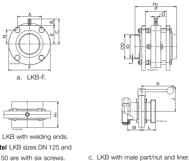
Fig. 1. Dimensions - valve.
