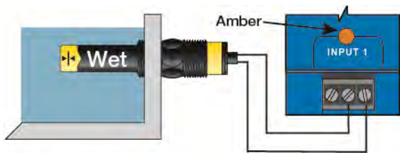
Single Switch Wet
