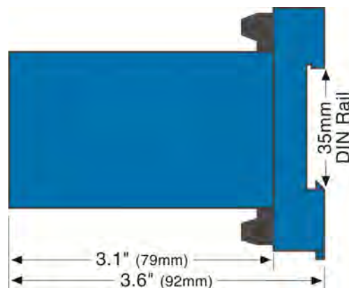
Side View - All Models
