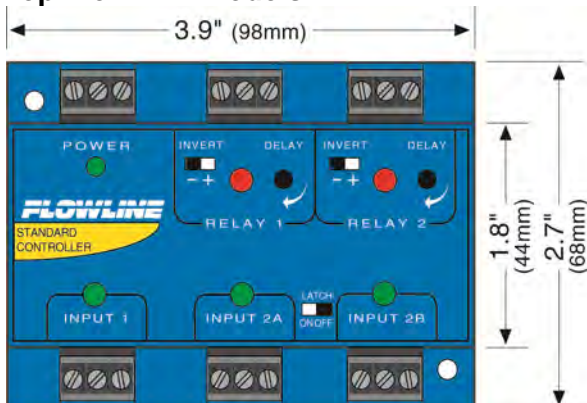
Top View - All Models
