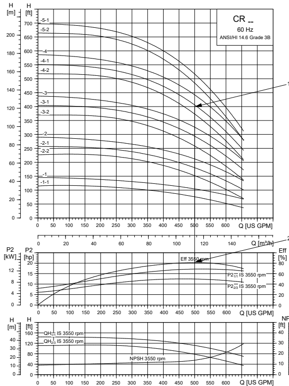
Example of a CR pump's duty point
