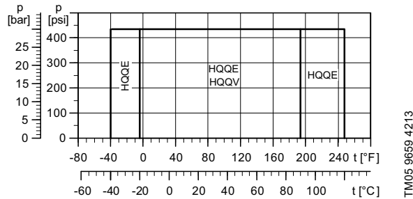
Fig. 44 Operating range of standard shaft seals for CRE 1s - CRE 20
