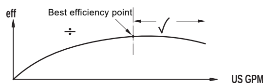
Fig. 49 Best efficiency
