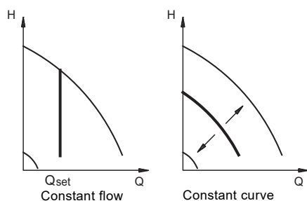
Fig. 3 E-pumps without a sensor
