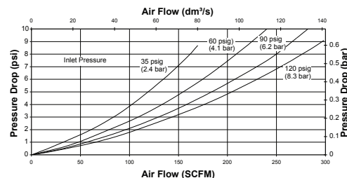
3/4" 3000 SERIES FILTER
