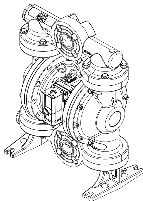
Model PD15X
