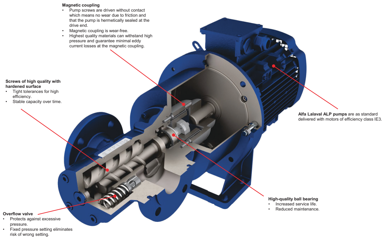
Figure 2. ALP magnetic coupling
