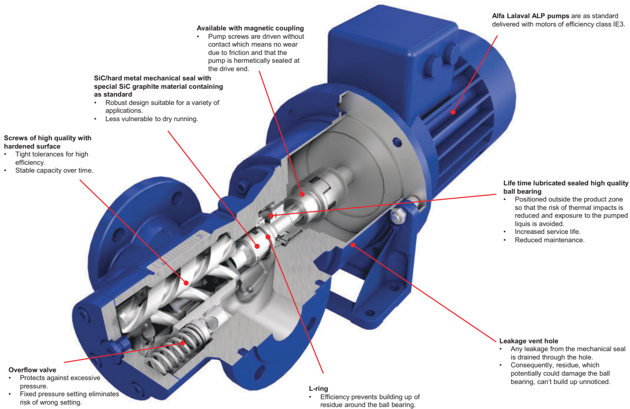
Figure 1. ALP mechanical coupling
