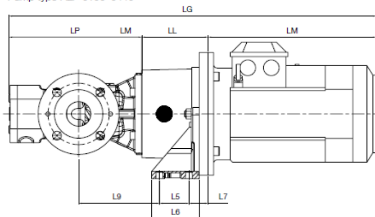
Pump type ALP 0100–0440
