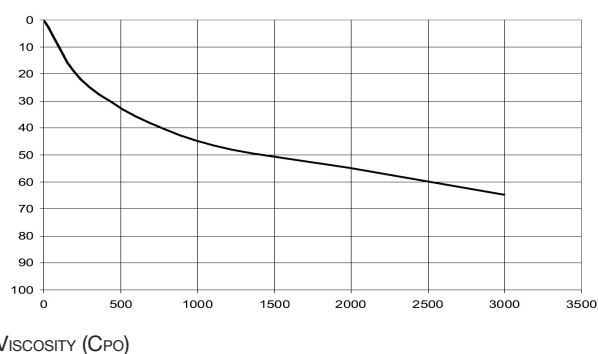
FLOW LOSS DUE TO VISCOSITY
