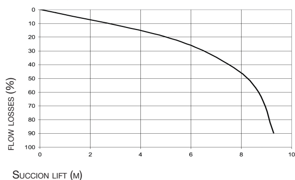
SUCCION LIFT LOSS
