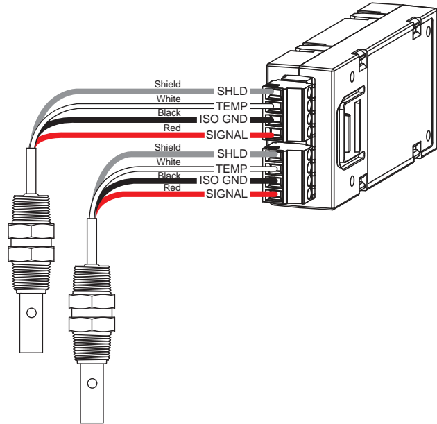
3-9950.394-2 Dual Channel Conductivity Module
