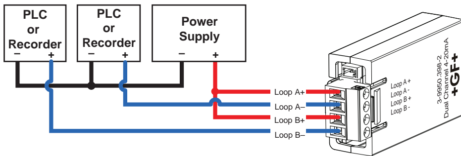
3-9950.398-2 Dual Channel 4 to 20 mA Module
