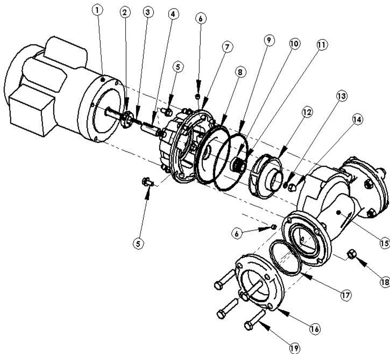
Figure 2 - Repair Parts Illustration
