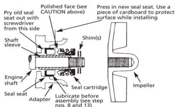
Figure 1A - Mechanical Seal Replacement
