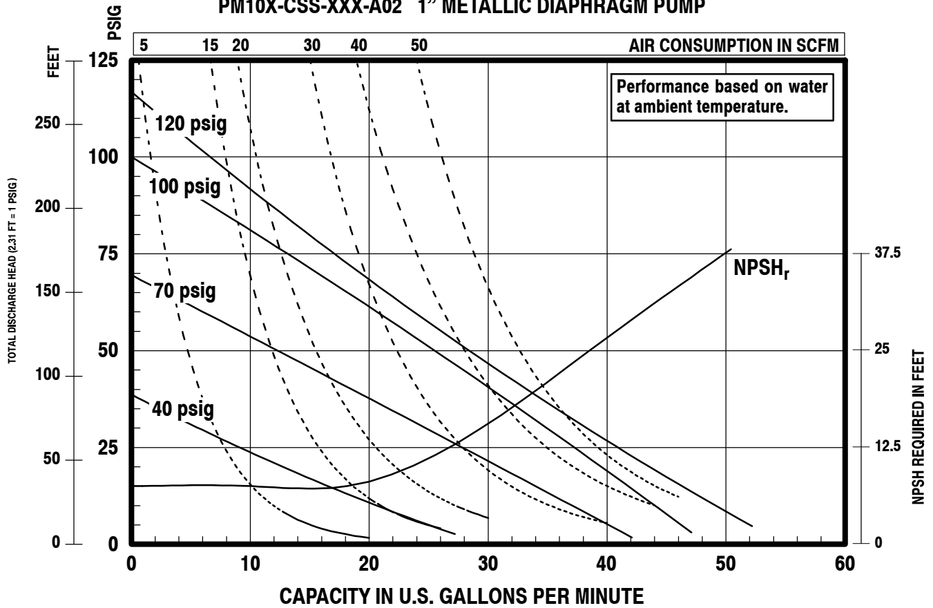
PM10X-CSS-XXX-A02 1" METALLIC DIAPHRAGM PUMP
