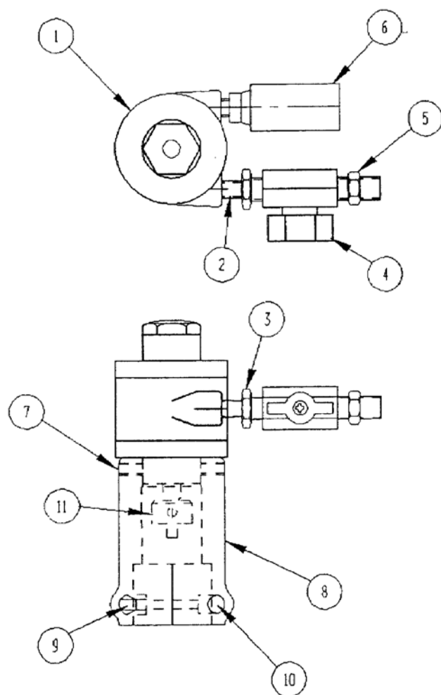
FILTER AND LUBRICATOR ASSEMBLY A100003
