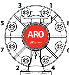
Torque Sequence
