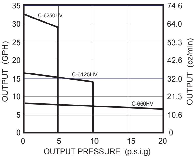
AC Powered Units Maximum Output vs. Pressure Curve
