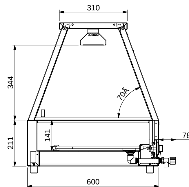
SECTION R-R
