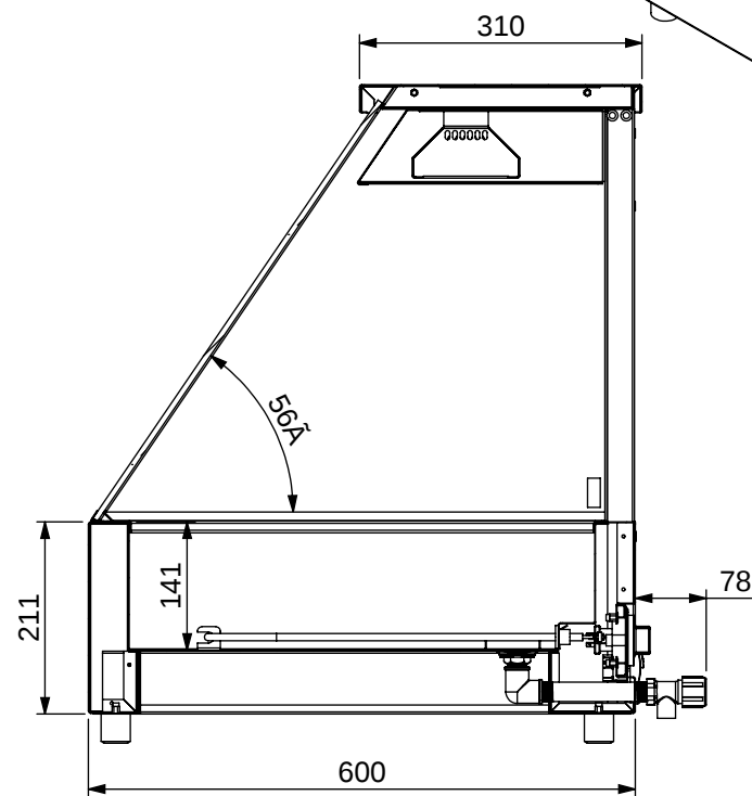
SECTION CF-CF
