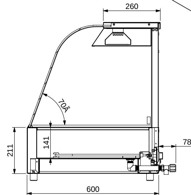
SECTION F-F
