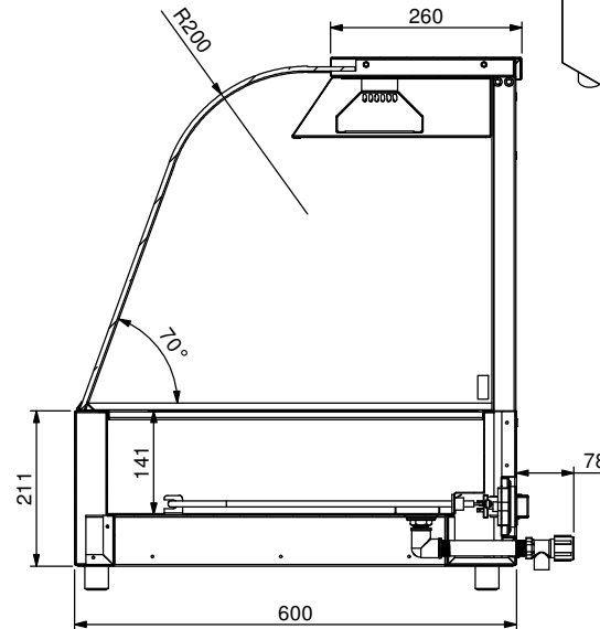
SECTION BK-BK
