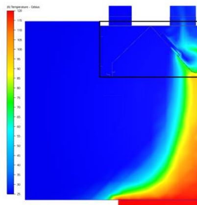
WITH ecoaircurtain™
