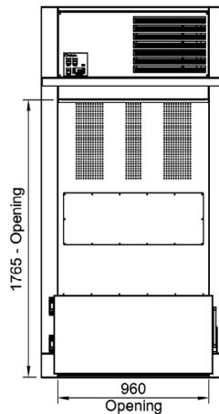
Front Elevation
