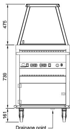
Front Elevation
