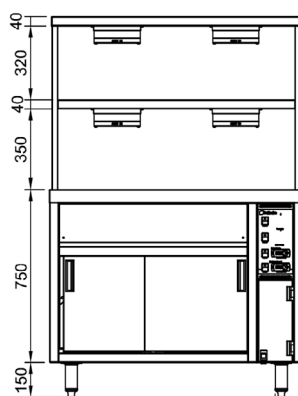
Front Elevation
