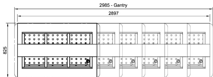
Plan View
