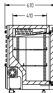
SIDE SECTION VIEW
