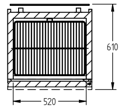
PLAN SECTION VIEW
