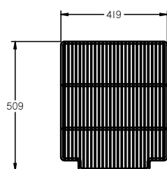
SHELF DETAIL
