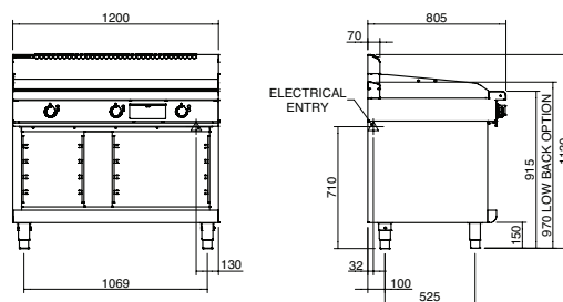
GP8120E-CB CABINET BASE
