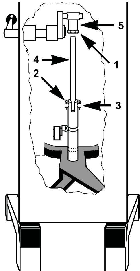
fig.7b Adjustment of bowl height:
