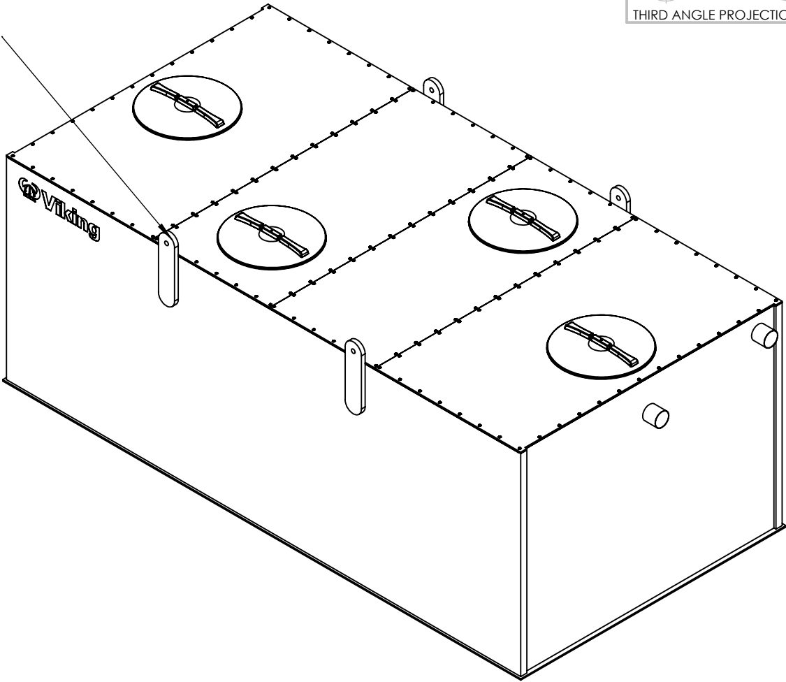
Lifting Lugs
