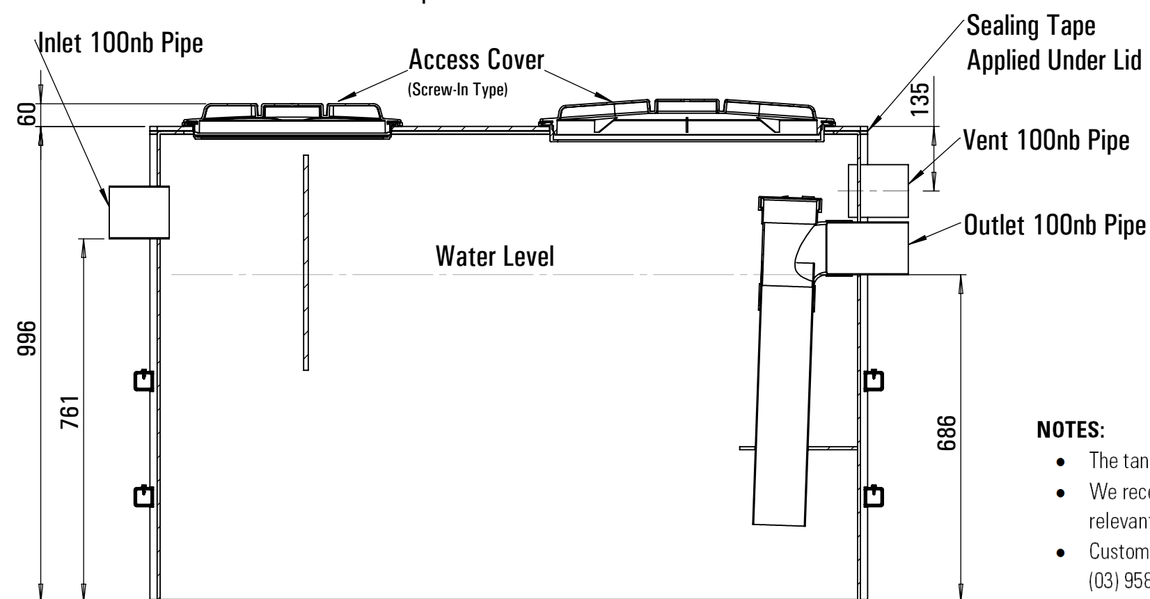
SECTION B-B
