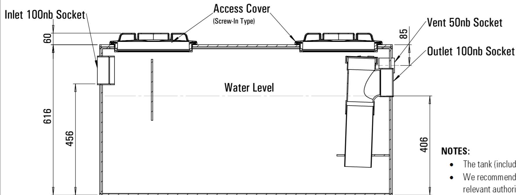
SECTION B-B
