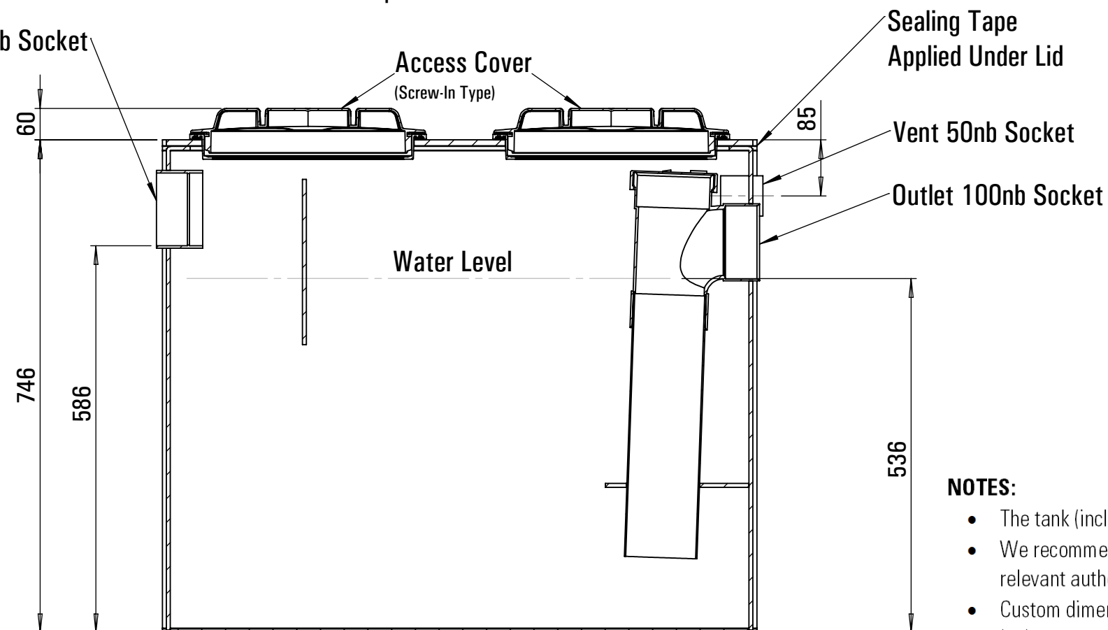
SECTION B-B
