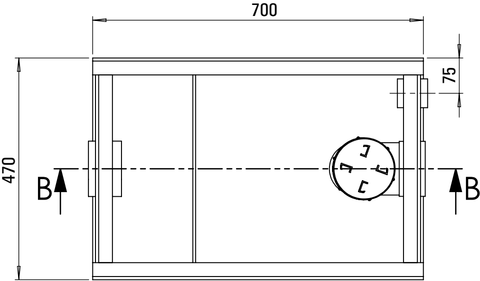
Top View without Lid
