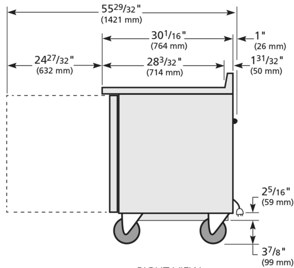
RIGHT VIEW
